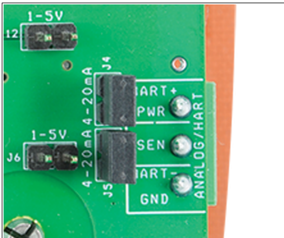
Figure 4: 4-20mA Jumper Terminals
