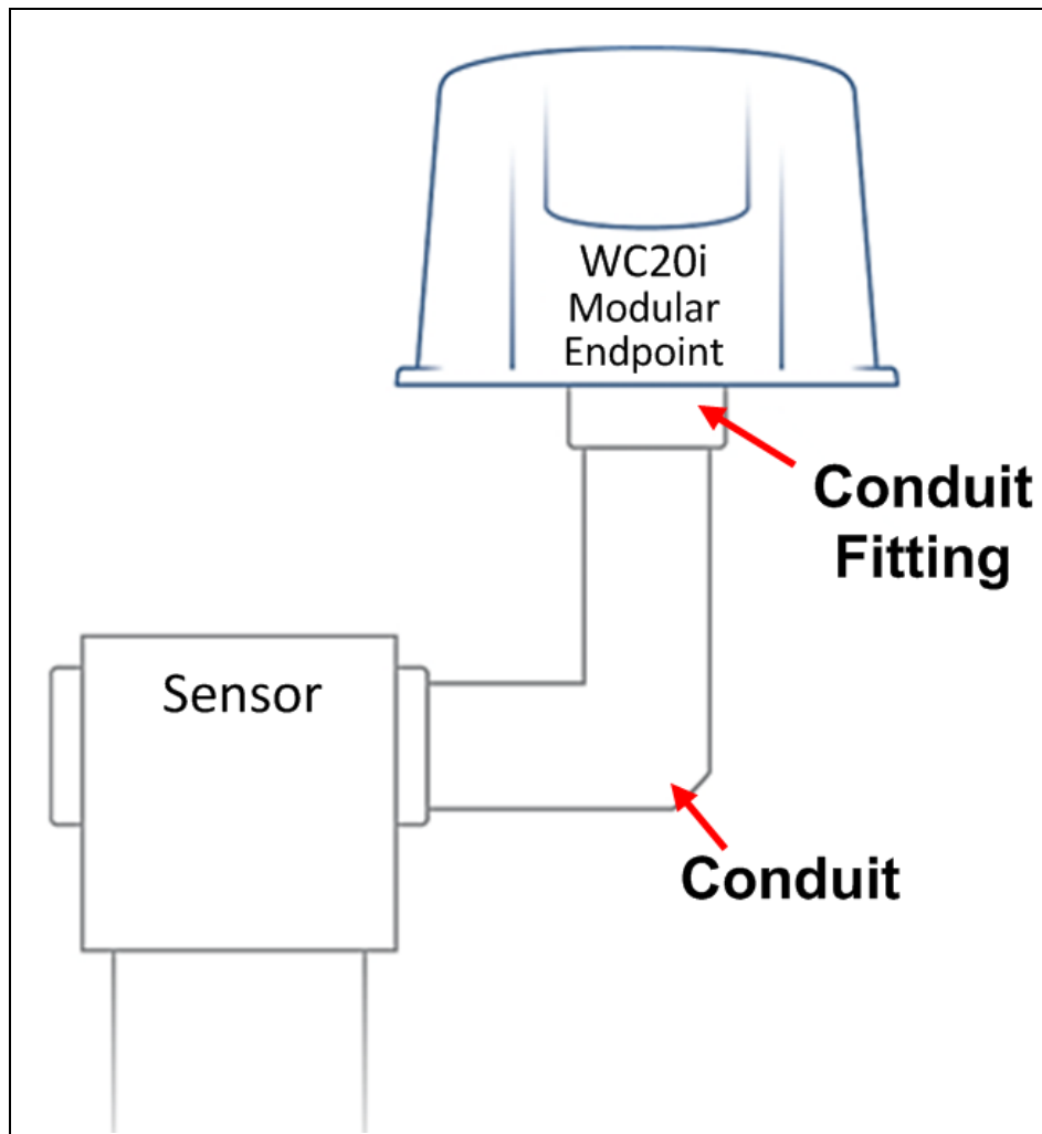
Figure 29: WC20i-AN or WC20i-AN-S Modular Endpoint Direct Mount
