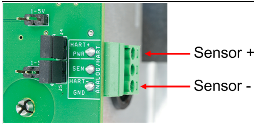
Figure 5: 4-20mA Sensor Connection
