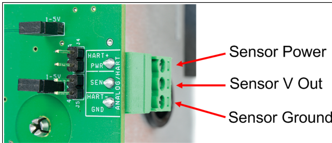
Figure 7: 1-5V Sensor Connection
