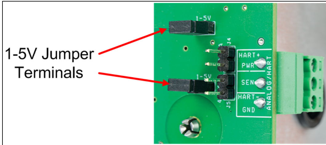
Figure 6: 1-5V Jumper Terminals
