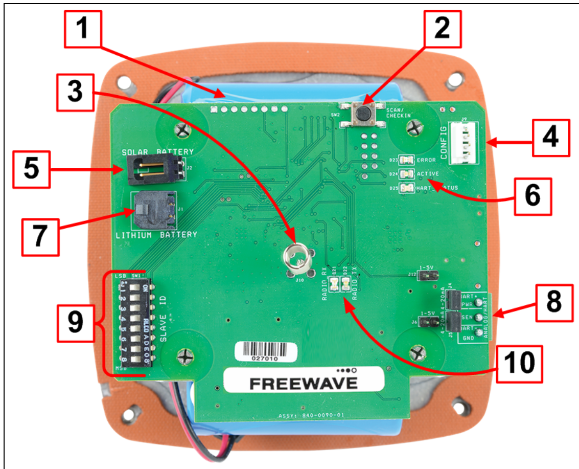
Figure 1: Internal Connections: WC20i-AN or WC20i-AN-S Modular Endpoint
