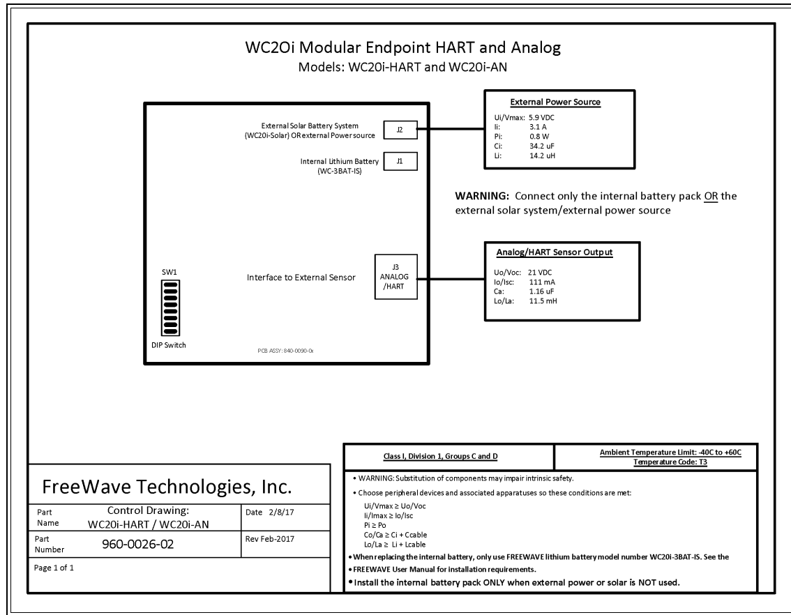
Figure 34: Control Drawing: WC20i-AN and WC20i-AN-S
